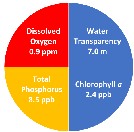
Figure 1. Lovell Lake Water Quality (2022)
